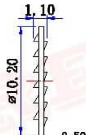
WASHER
